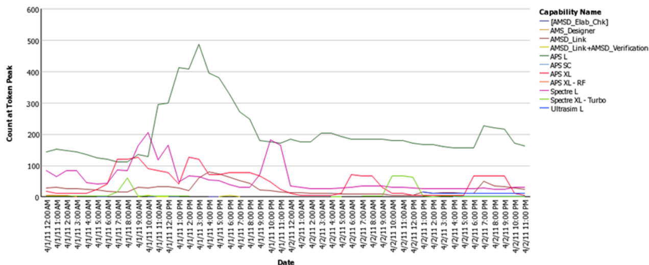
Figure 5-12: Part of a Token-Capability Peak Usage report.
